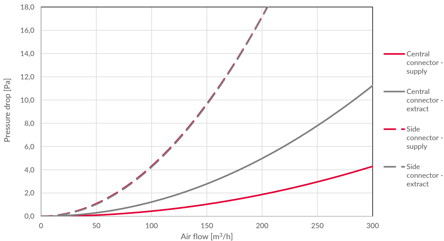
HEATPEX ARIA CONNECT 10x75 Distribution box
